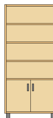
STM-200-30T 90 X 48 X 200 H cm
